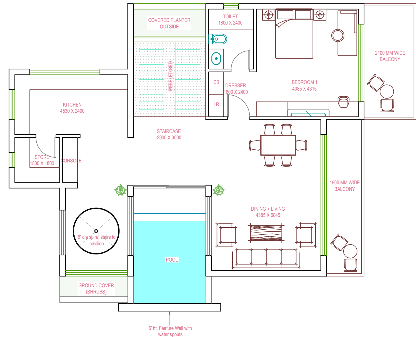
LOWER GROUND FLOOR PLAN CARPET AREA 180 SQM.
