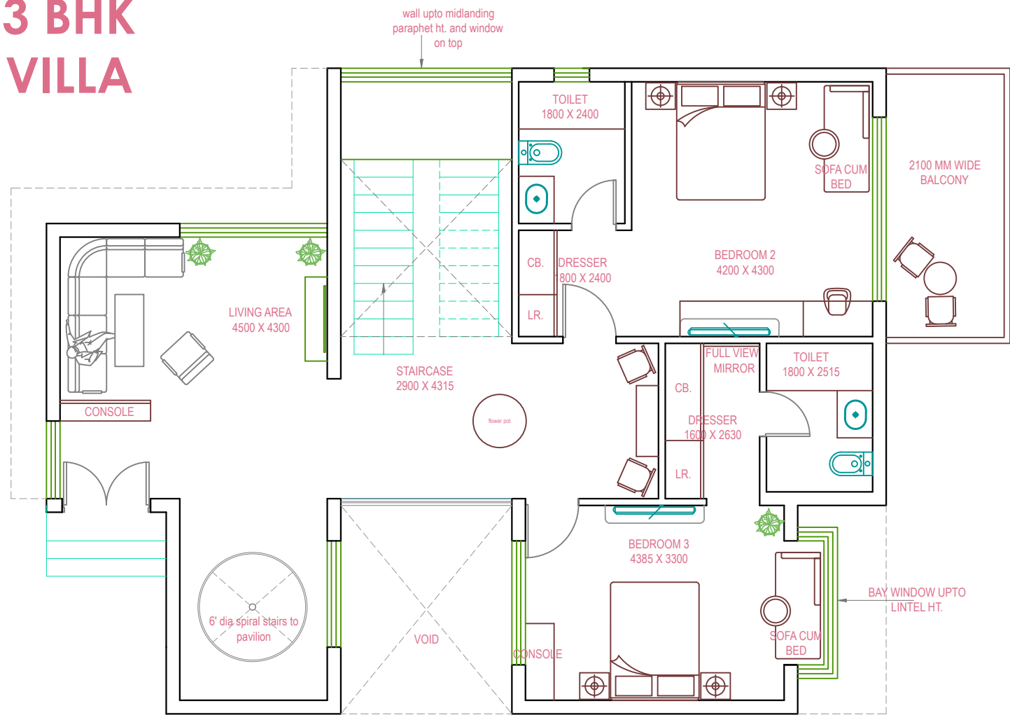
GRUND FLOOR PLAN ENTRY LEVEL
